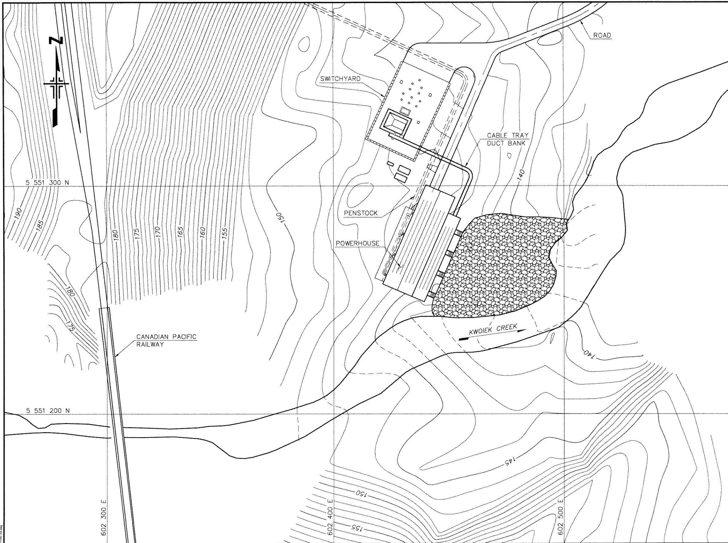
PLAN VIEW 1:1000
